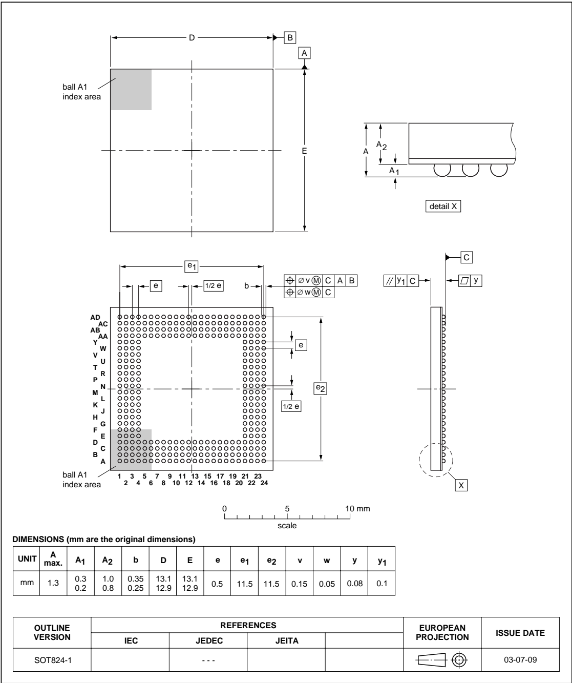
LFBGA320: plastic low profile fine-pitch ball grid array package; 320 balls; body 13 x 13 x 0.9 mm SOT824-1
